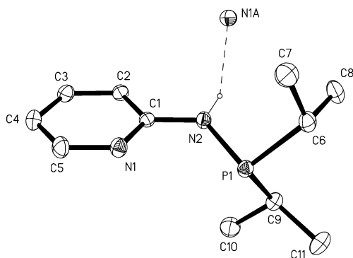
Figure 1. Molecular structure of PN- i Pr showing 50% displacement ellipsoids. Only N-bonded hydrogen is shown. Selected distances and angles (Å, deg): P1–N2 1.721(1), P1–C6 1.857(1), P1–C9 1.856(1), N1–C1 1.339(1), N1–C5 1.346(1), N2–C1 1.382(1), C1–C2 1.413(1), C2–C3 1.381(1), C3–C4 1.393(1), C4–C5 1.381(1); P1...N1 2.999(1); P1–N2–C1–N1–17.9(1); hydrogen bond N2–(H2n)...N1A 3.203(1).
