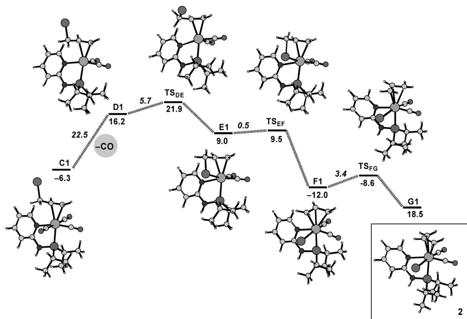
Figure 7. Profile of the B3LYP potential energy surfaces (free energies in kcal/mol) for the conversion of C1 to the final \eta^3 -allyl complex G1 .
