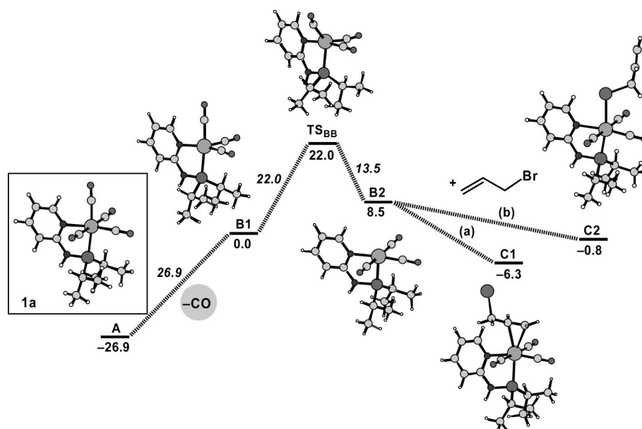
Figure 6. Profile of the B3LYP potential energy surfaces (free energies in kcal/mol) for the formation and interconversion of tricarbonyl complexes B1 and B2 and addition of allyl bromide via (a) an initial \eta^2 \pi complex and via (b) a direct Br attack to give C1 and C2 , respectively.
