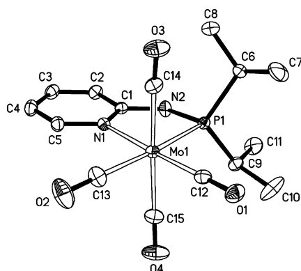
Figure 2. Molecular structure of 1b showing 50% displacement ellipsoids. H atoms omitted for clarity.
