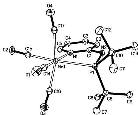
Figure 3. Molecular structure of 1c (50% displacement ellipsoids, H atoms omitted for clarity). The Figure emphasizes the steric effect of the bulky t\text{Bu} groups on the two carbonyl groups C16–O3 and C17–O4. P1 deviates by -0.315(2) Å from the least-squares plane of the pyridine ring, Mo1 by 0.152(2) Å. \text{P1-N2-C1-N1} 15.8(1)°.
