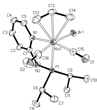
Figure 5. Molecular structure of 2 (50% displacement ellipsoids, H atoms omitted for clarity). Selected bond lengths and angles (Å, deg): Mo1–C16 1.935(2), Mo1–C15 1.957(2), Mo1–C13–2.223(2), Mo1–C12–2.328(2), Mo1–N1 2.329(2), Mo1–C14 2.351(2), Mo1–P1–2.5215(5), Mo1–Br1–2.6863(3) Å; N1–Mo1–P1 75.20(4), P1–Mo1–C13 163.46(5).
