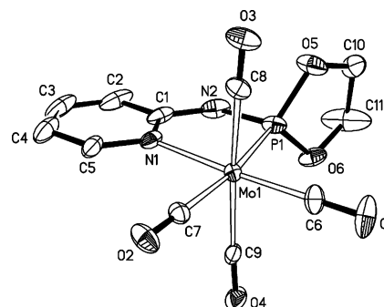
Figure 4. Molecular structure of 1d . This complex approaches a non-crystallographic C_s symmetry.
